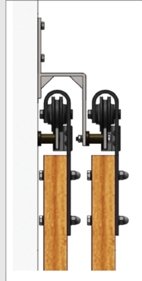
BYPASS RAIL BRACKET (Stainless Steel option shown)
